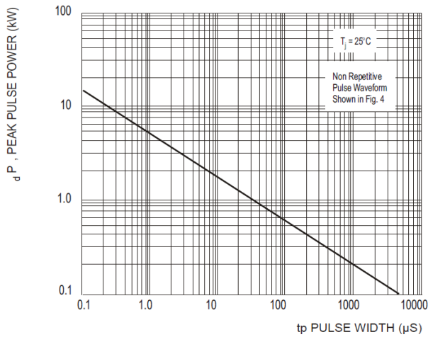
Fig. 3 Pulse rating curve
