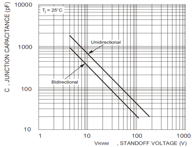
Fig. 2 Typical Total Capacitance
