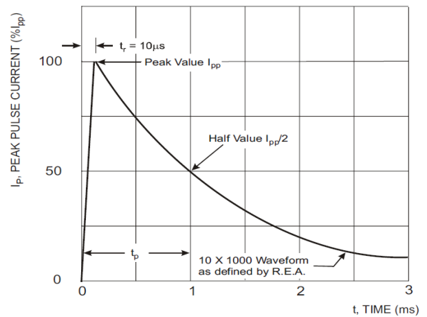
Fig. 4 Pulse Waveform
